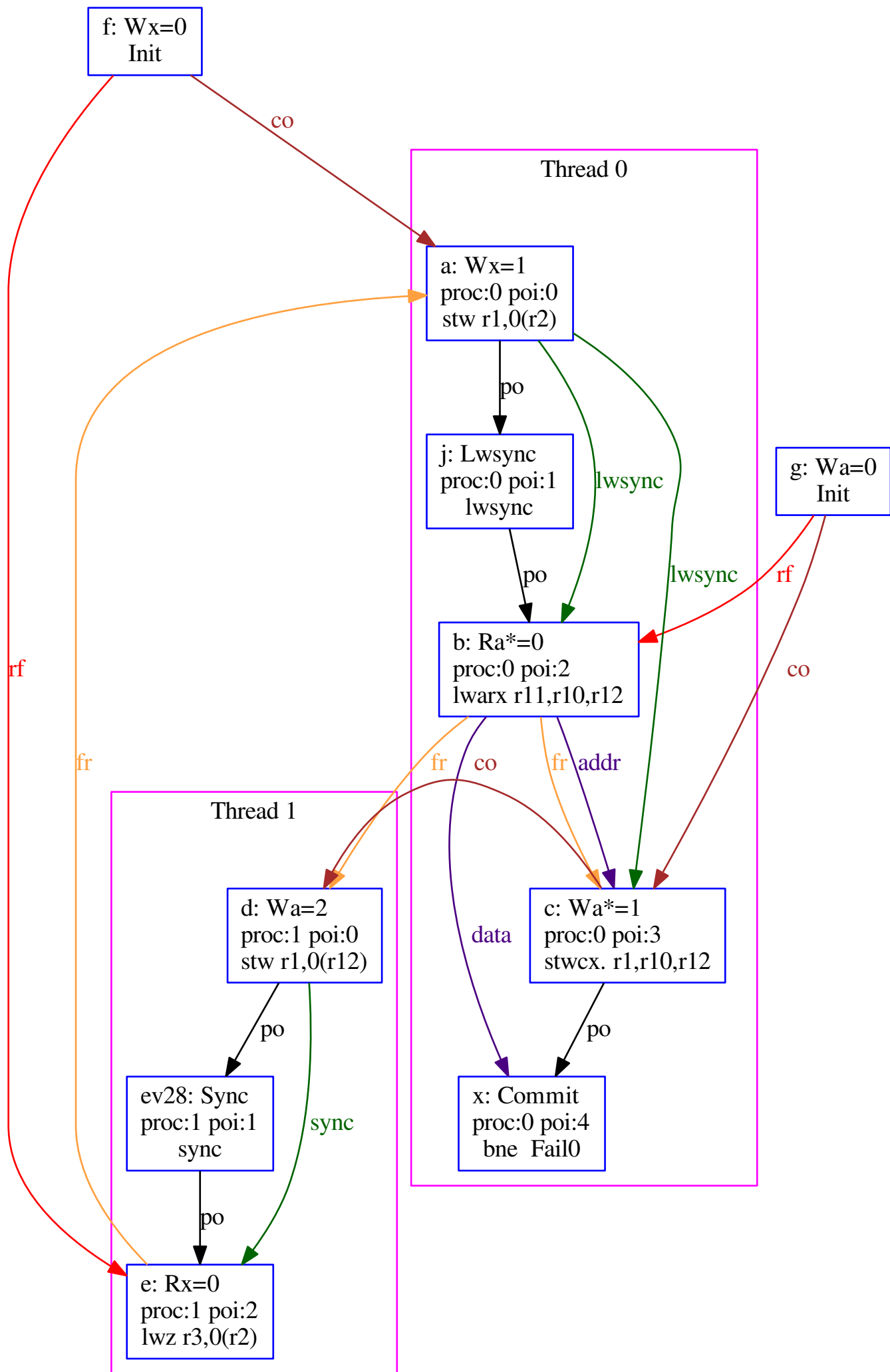
Test SB+lwsync-RMW2-lwsync+st-sync-leading, Generic(PPC)
