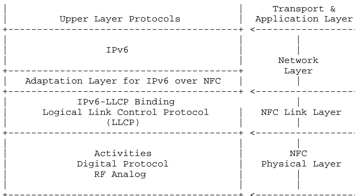
Figure 3: Protocol Stacks for IPv6 over NFC
