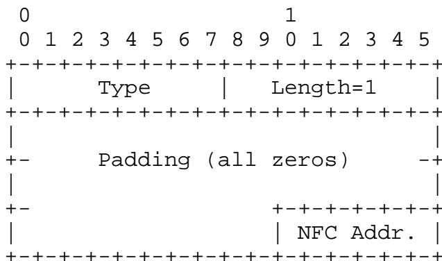
Figure 9: Unicast address mapping
