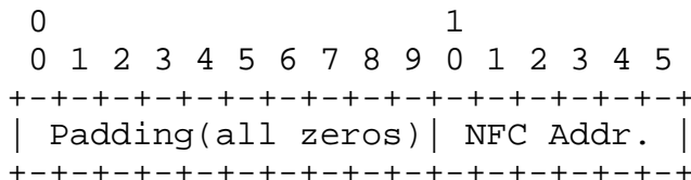
Figure 8: NFC short address format
