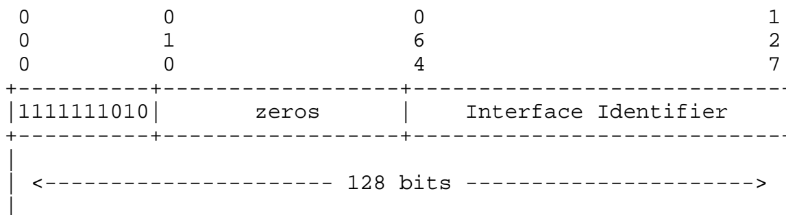
Figure 5: IPv6 link-local address in NFC
