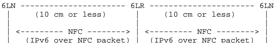
Figure 11: Isolated NFC-enabled device network
