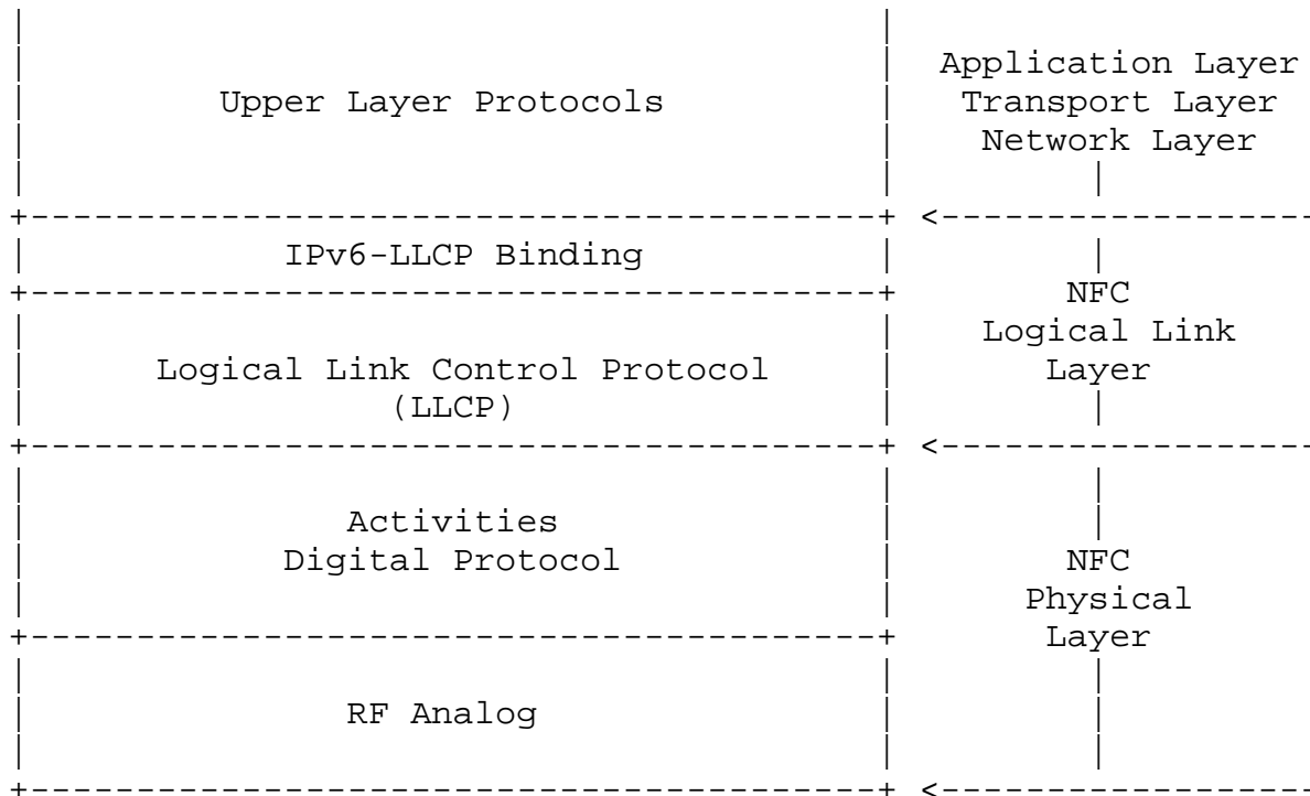
Figure 1: Protocol Stacks of NFC
