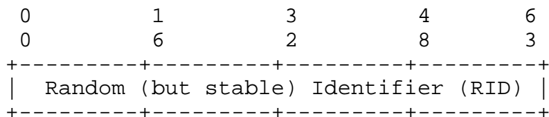
Figure 4: IID from NFC-enabled device
