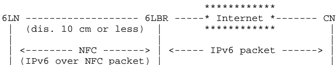
Figure 10: NFC-enabled device network connected to the Internet
