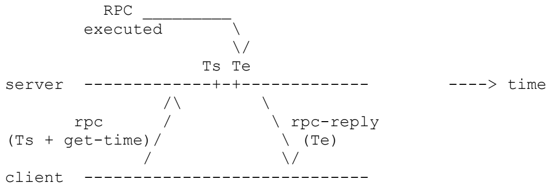
Figure 3 Scheduling and Reporting
